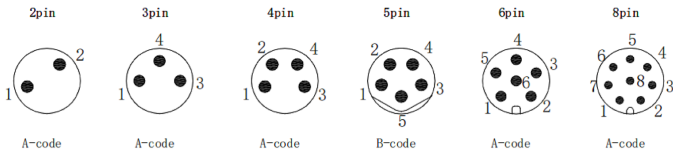
Pin assignment front view/针位分布前视图
